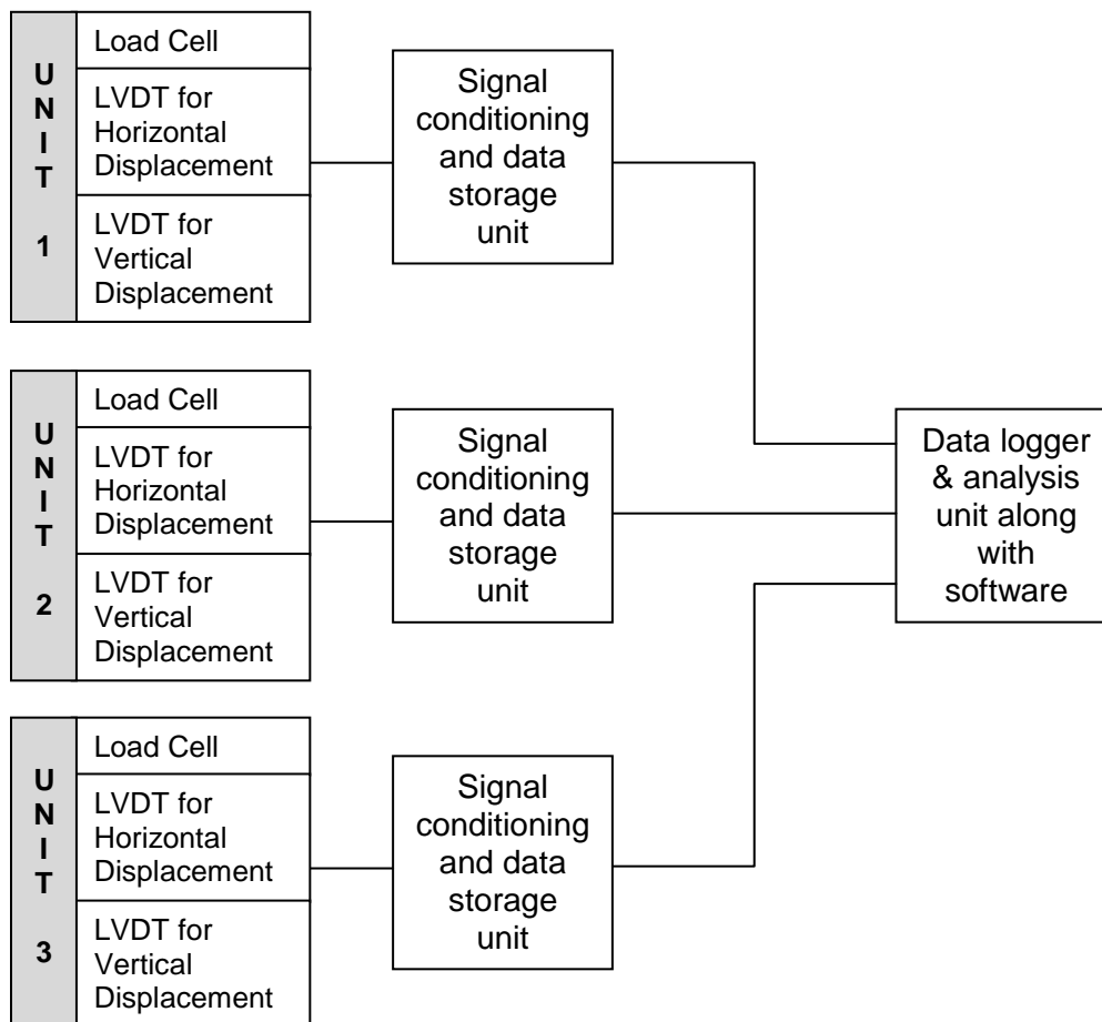
Fig. 1 Schematic Representation of Direct Shear Apparatus (3 Units) with Signal Conditioning and Data logger units
