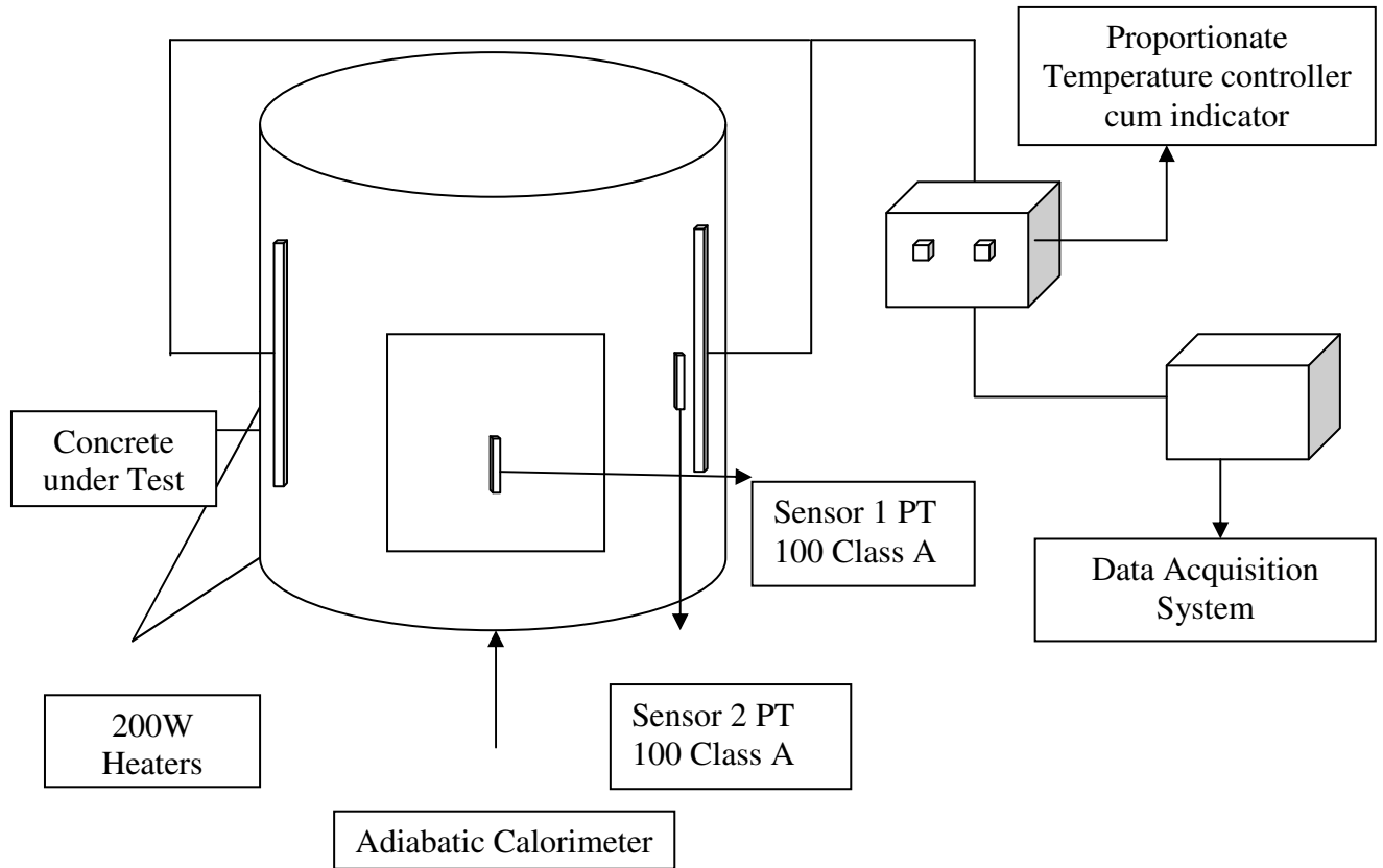
Systematic diagram of Complete Set up
