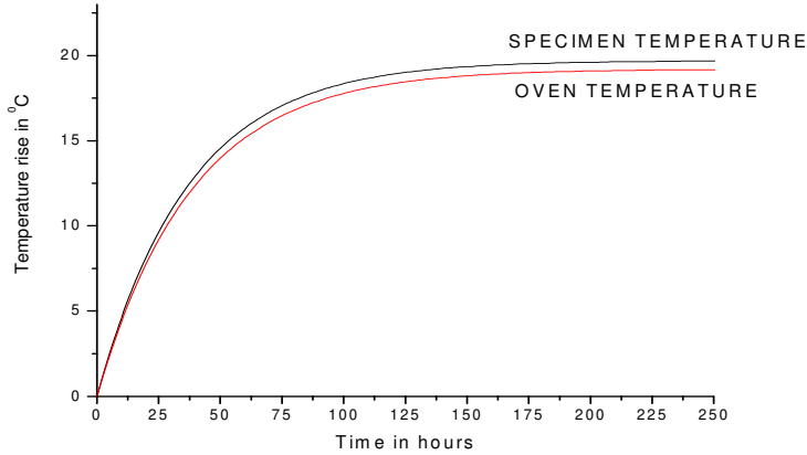
GRAPH A - TYPICAL ADIABATIC TEMPERATURE RISE CURVE
