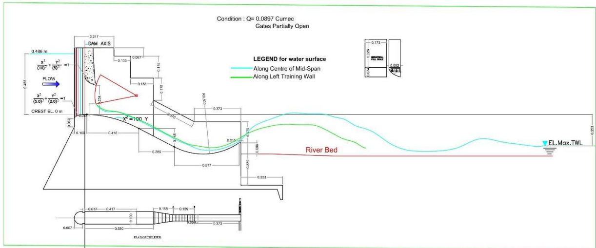
Figure 2: Design Sketch of Spillway and Downstream river bed
