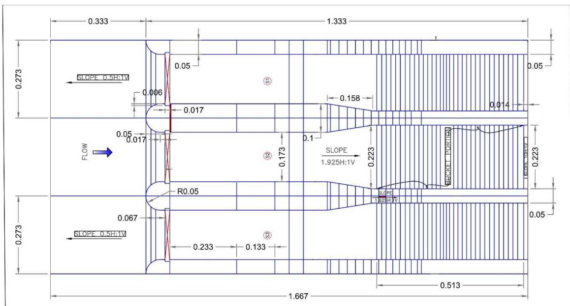
Figure 3: Design Sketch of Spillway Plan
