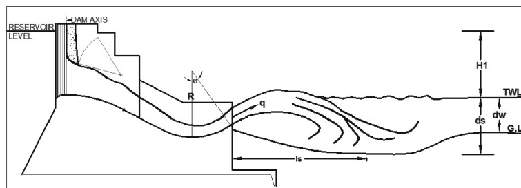
Figure 1: Scour downstream of the ski-jump bucket spillway
