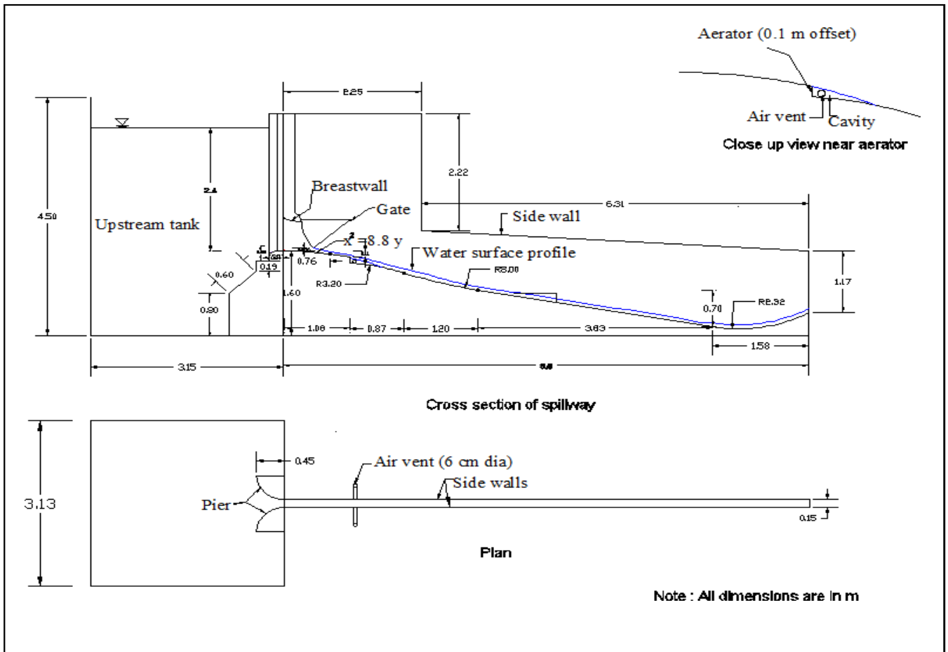
Figure 1 : Definition sketch of the spillway
