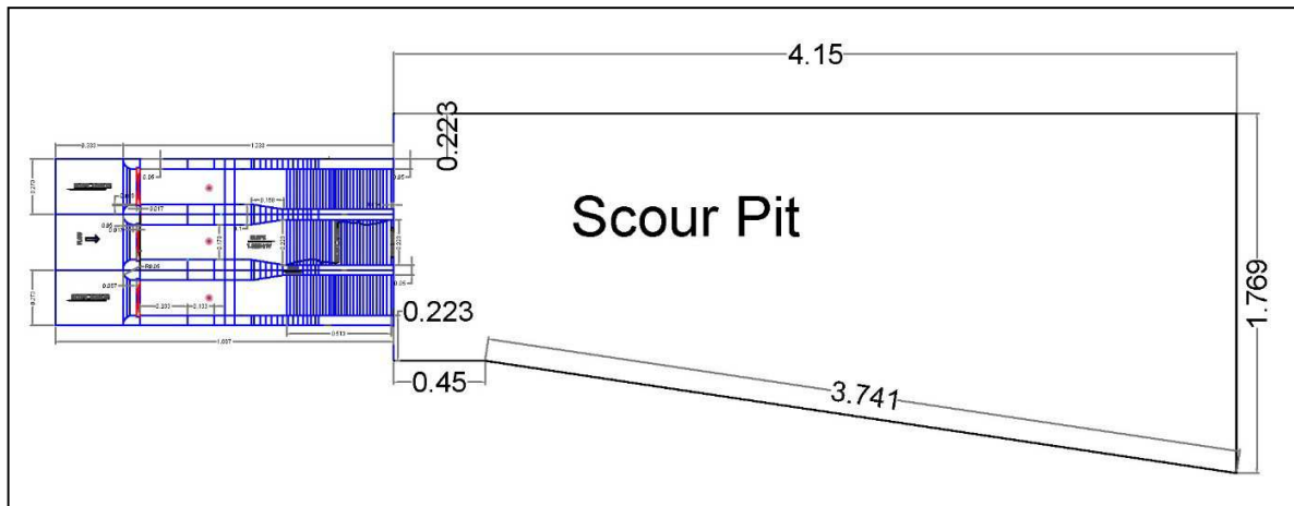
Figure 4: Design Sketch of Spillway with Scour Pit in Plan
